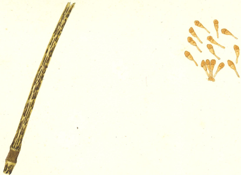
Puccinia graminis. Pers.
