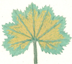
Uromyces Alchemillae (Pers.) Uredo ( Trichobasis (Uredo) alchemillae (Pers.))
